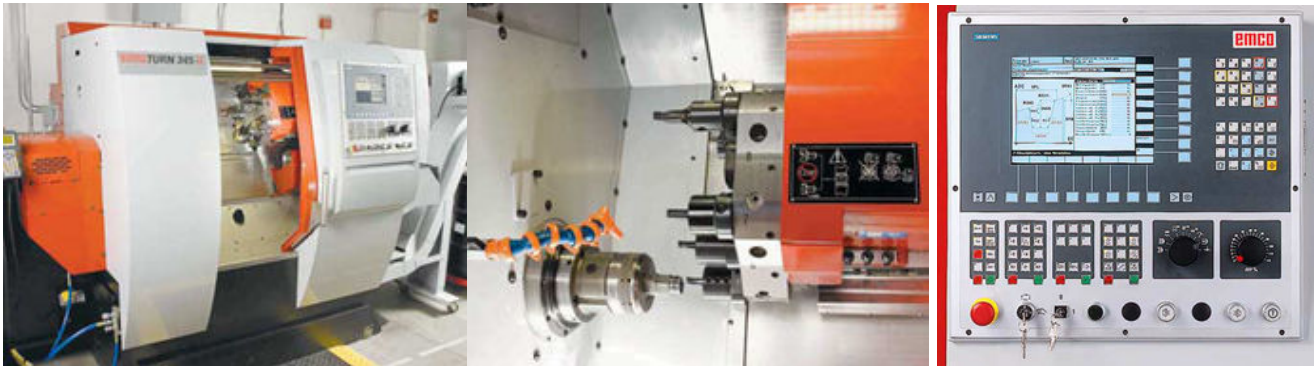
Emco Maier EMCOTURN 345-II (Now called the MaxxTurn45 w/ Siemens 840D), a CNC lathe with 12-position tool changer, six driven tools and a 45mm (1.77") diameter max. barstock feed. Siemens SINUMERIK 810D CNC can operate six axes and two spindles.
